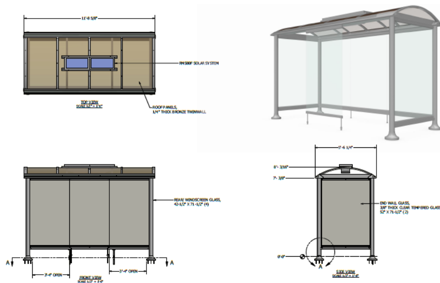
Figure 3: Existing standard shelter as deployed throughout CATA’s system
